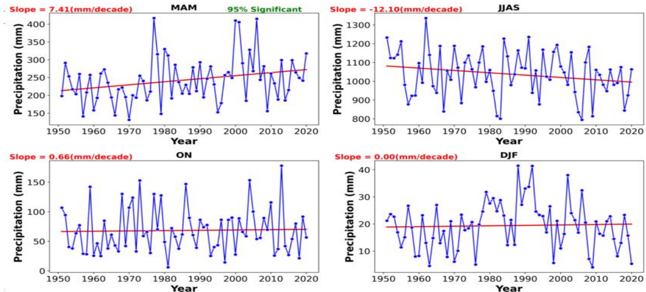
Figure 6 Timeseries (blue) along with trend lines (red). Significant trends are highlighted at 95% significance level using MK test.
