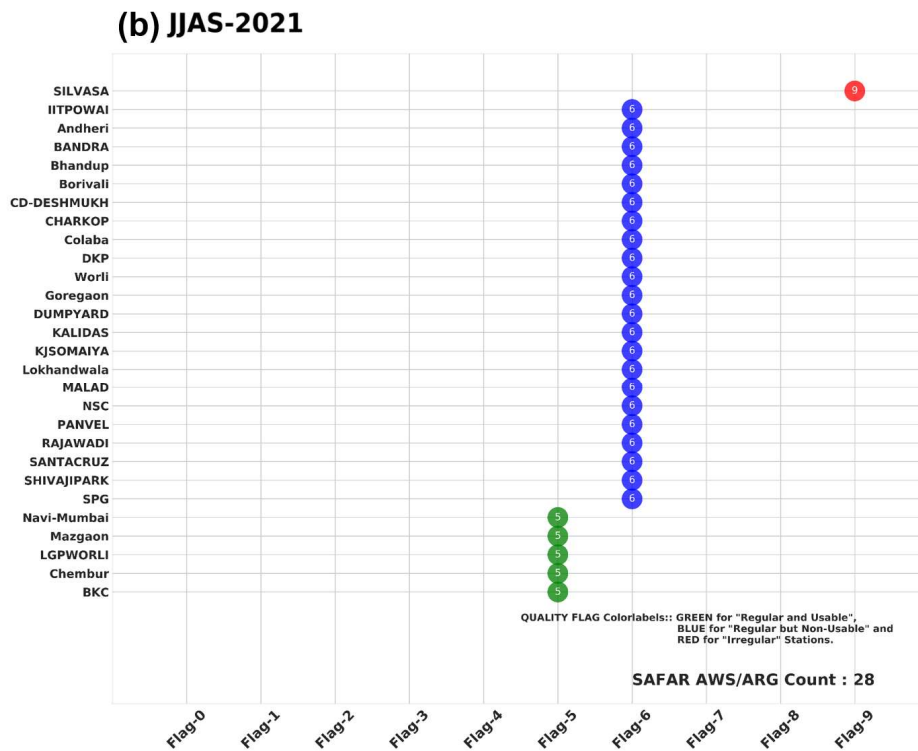
Fig. 13B. Status of each SAFAR-maintained ARG stations based on the Quality Flags assigned to those stations reporting rainfall observations during monsoon (JJAS) months of (a) 2020 and (b) 2021.
