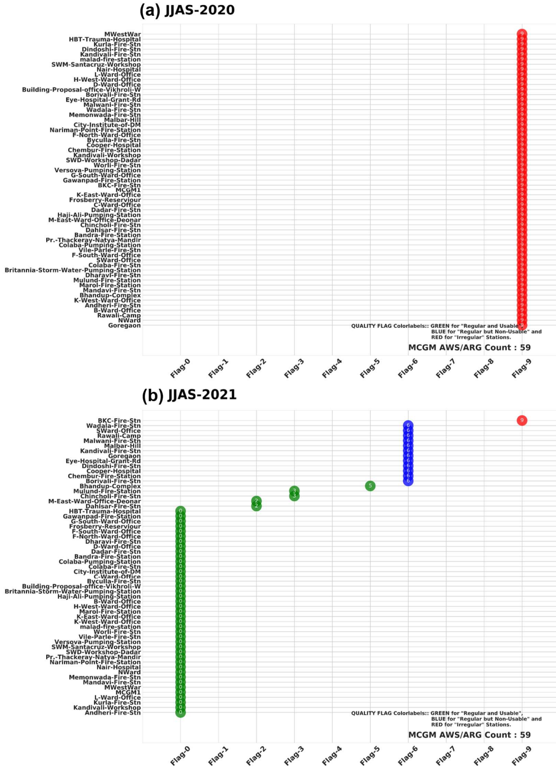
Fig. 11B. Status of each MCGM-maintained ARG stations based on the Quality Flags assigned to those stations reporting rainfall observations during monsoon (JJAS) months of (a) 2020 and (b) 2021.
