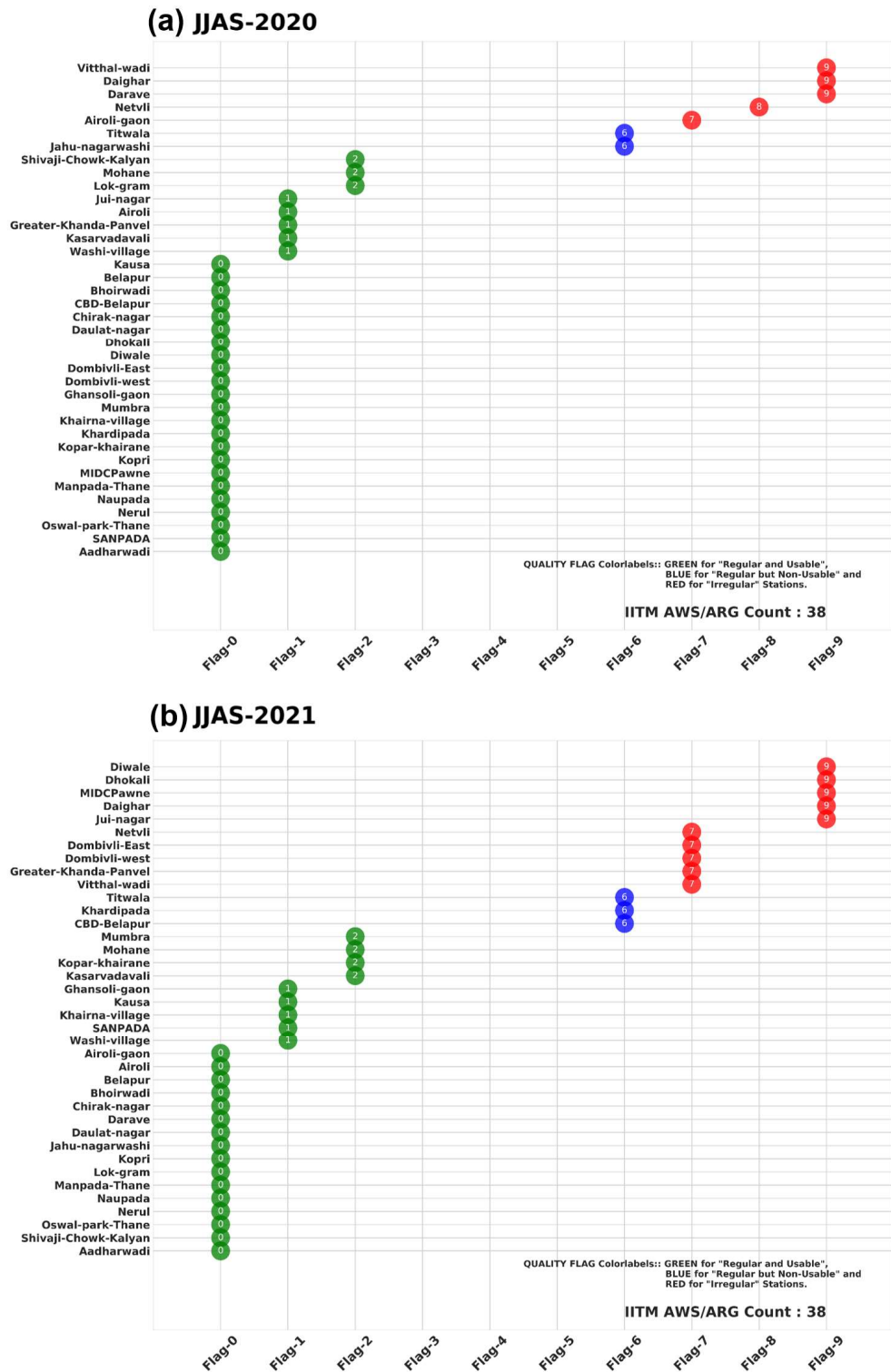
Fig. 10B. Status of each IITM-maintained ARG stations based on the Quality Flags assigned to those stations reporting rainfall observations during monsoon (JJAS) months of (a) 2020 and (b) 2021.
