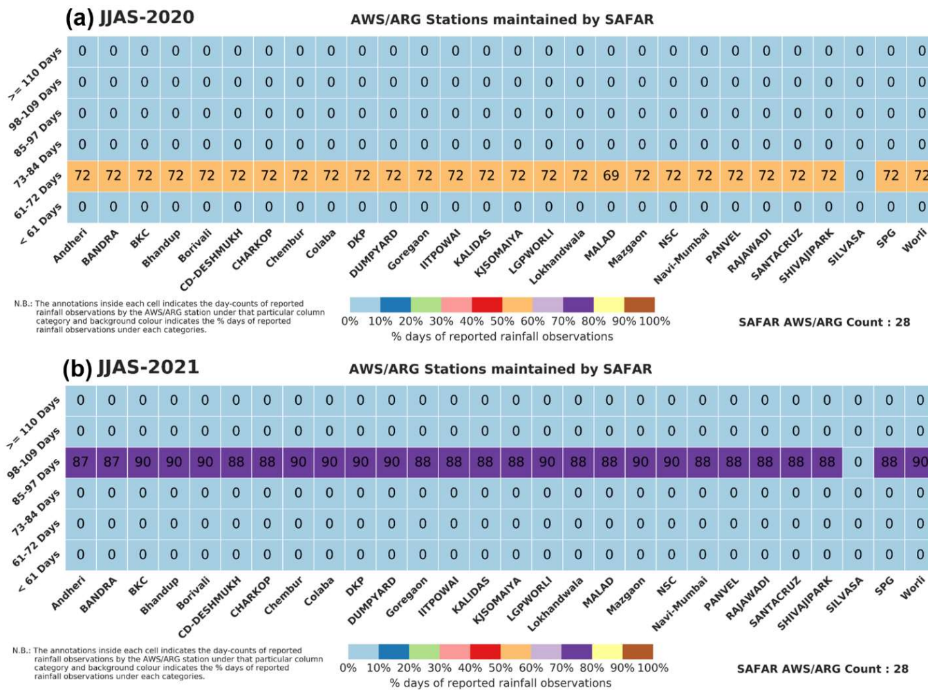
Fig. 13A. Heatmap statistics, for each ARG sites, based on the percentage count as well as the reported count of rainfall observations by ARG stations as maintained by SAFAR during monsoon (June-September, JJAS) months of (a) 2020 and (b) 2021.
